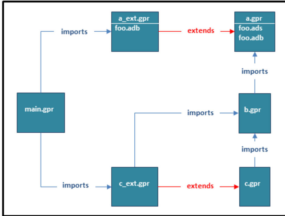
Fig. 2.1: Example of Source File Ambiguity from imports/extends Violation
